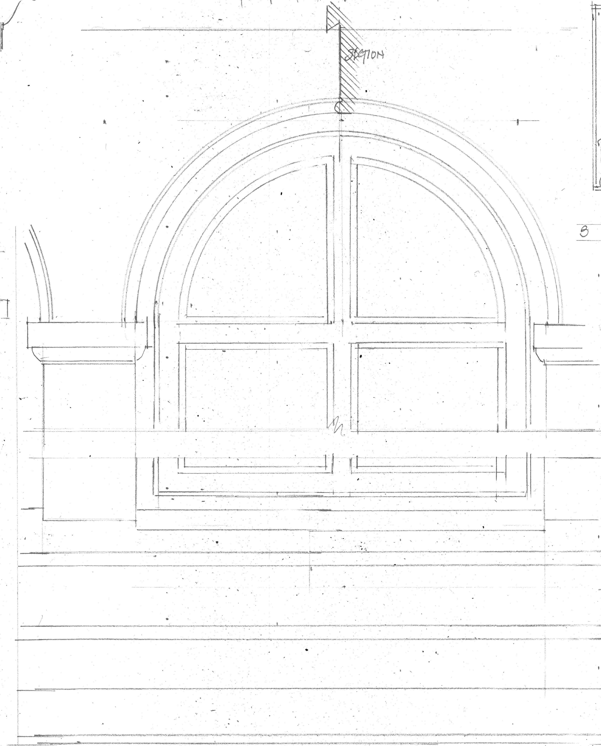
PART ELEVATION ORIEL
