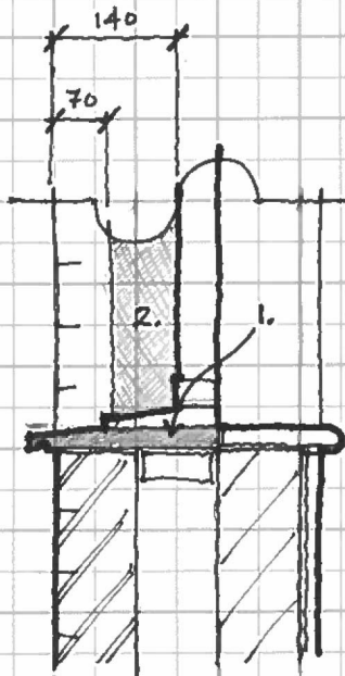
SECTION 1:10
