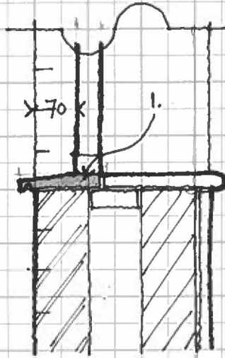
SECTION 1:10
